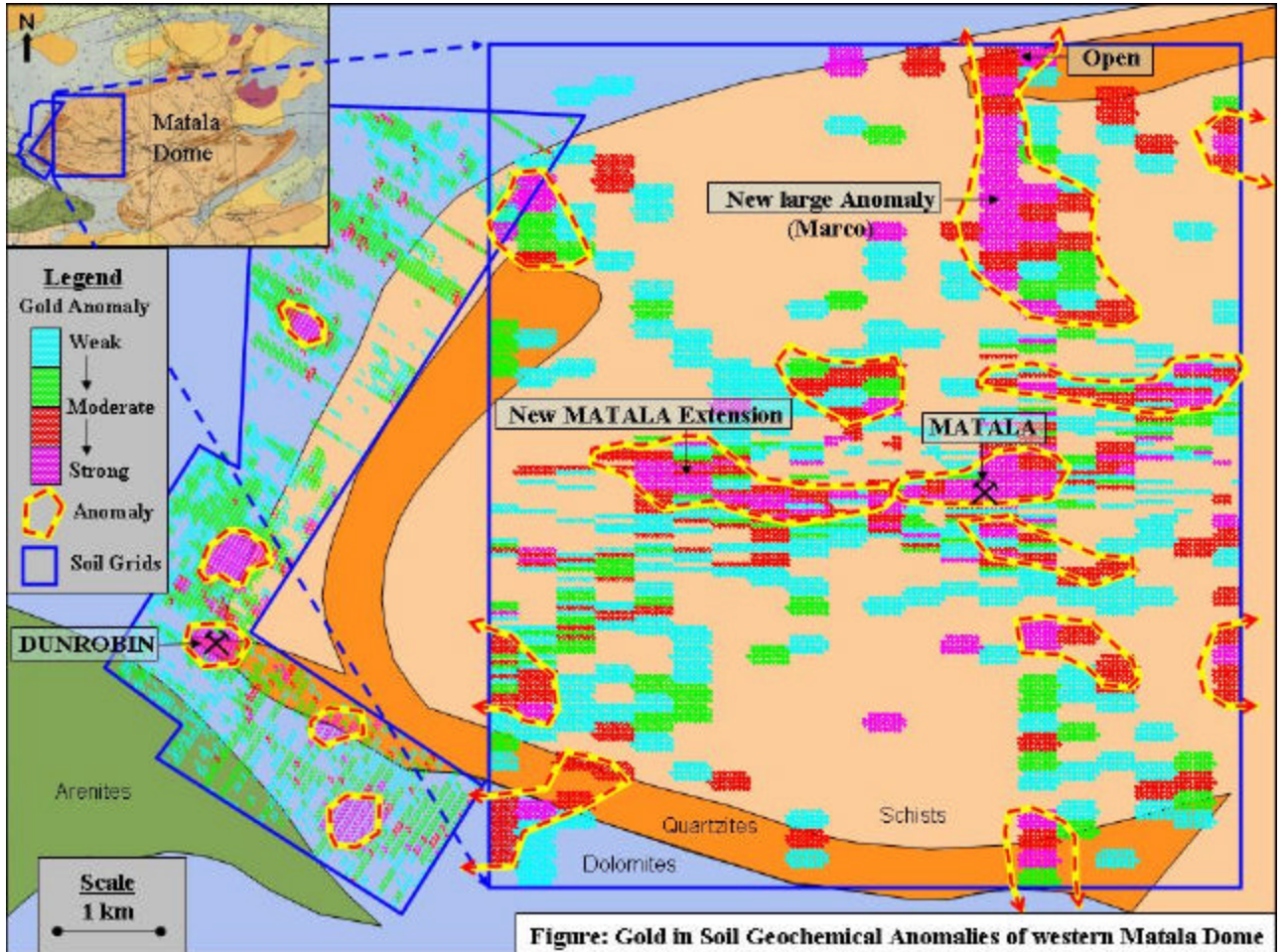
Figure1 – The new Marco Anomaly shown within context of the Matala Dome structure, Zambia.
