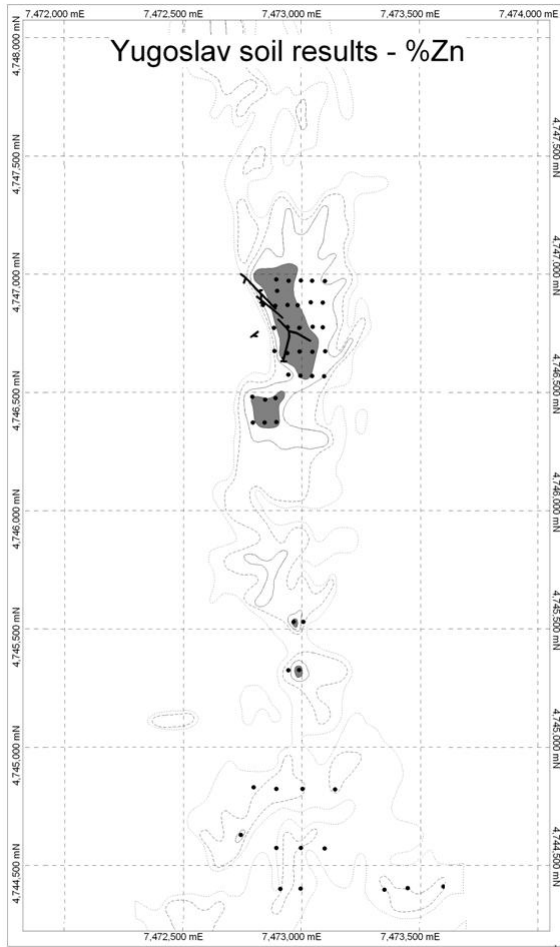
Figure 1. Soil geochemical results – zinc (contours 0.05, 0.1, 0.2, and 0.5%); Lydian's orientation soil lines positions and trace of underground adits included. (grid squares are 500m by 500m).
