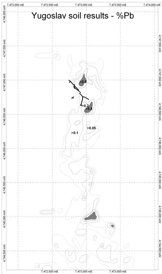
Figure 2. Soil geochemical results - lead (contours 0.05, 0.1, 0.2, and 0.5%). Lydian's orientation soil lines positions based on Yugoslav Zn contours (Figure 1 - left).
