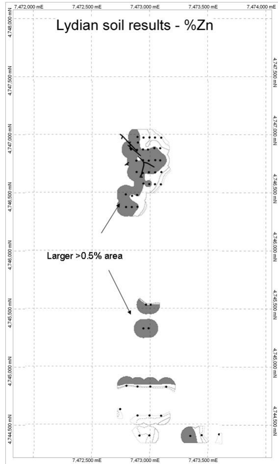
Figure 1. Soil geochemical results – zinc (contours 0.05, 0.1, 0.2, and 0.5%); Lydian's orientation soil lines positions and trace of underground adits included. (grid squares are 500m by 500m).
