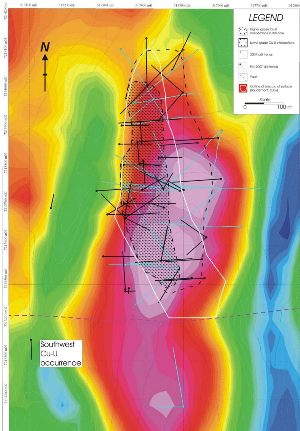
Figure 3: Map showing all drilling at the Igor property (including historical), and an outline of interpreted low grade and high grade Cu-U mineralization overlaying a gravimetric image. An outcropping breccia is also shown.
